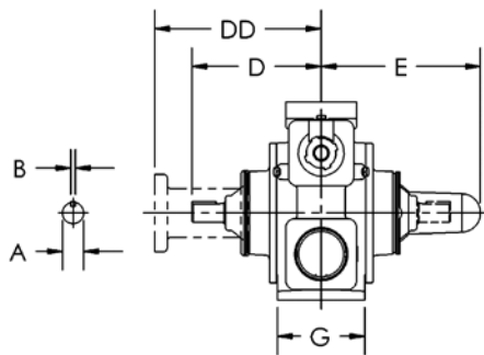
Keyed Shaft and Hydraulic Drive Option
