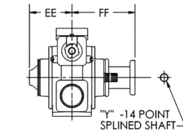
Splined Shaft Hydraulic Drive Option (left hand rotation only)
